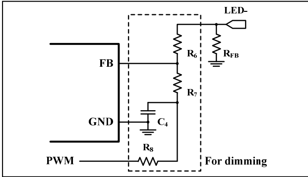
Figure 18 RC PWM Dimming
