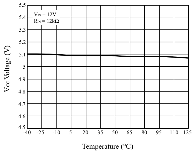
Figure 13 Temperature vs. V CC
