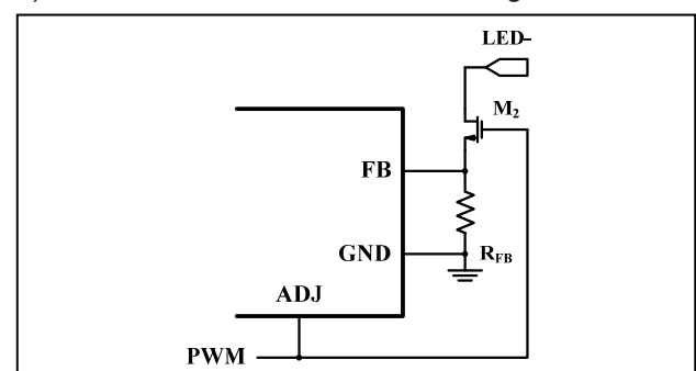
Figure 17 External PWM Dimming
